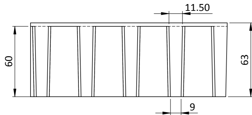
ELEVATION VIEW
